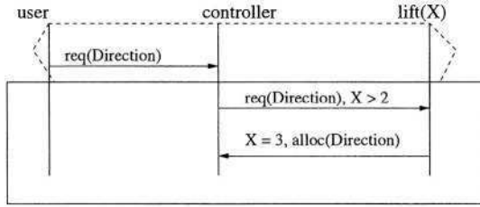
Fig. 4. A chart with universally quantified control variable ( X in this case)
