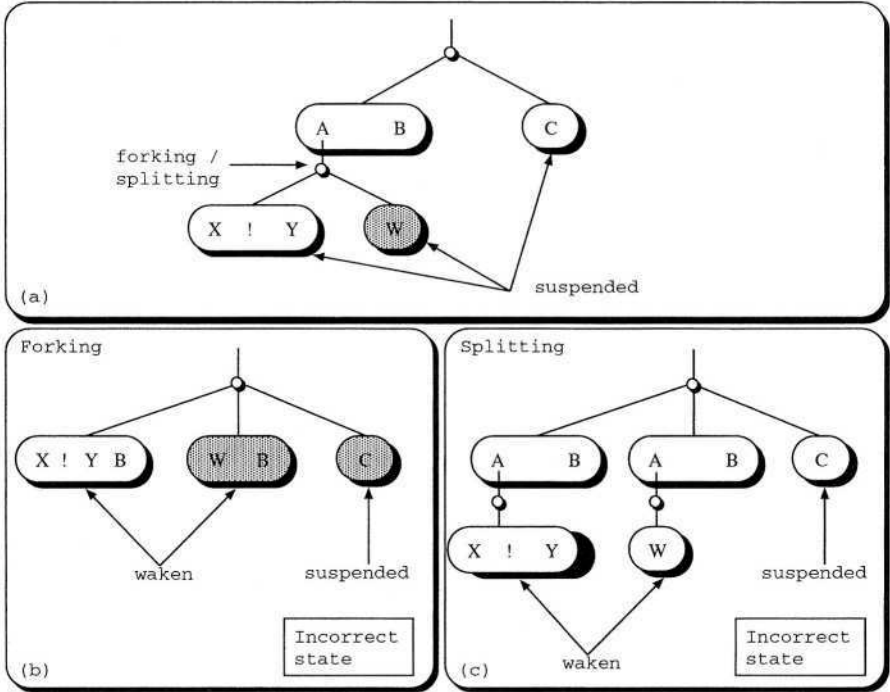
Fig. 6. Incorrect use of fork/splitting and cut.
