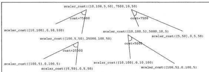
Fig. 2. Recursion tree for computing scalar_cost([10,100,5,50], V, 10, 50)
