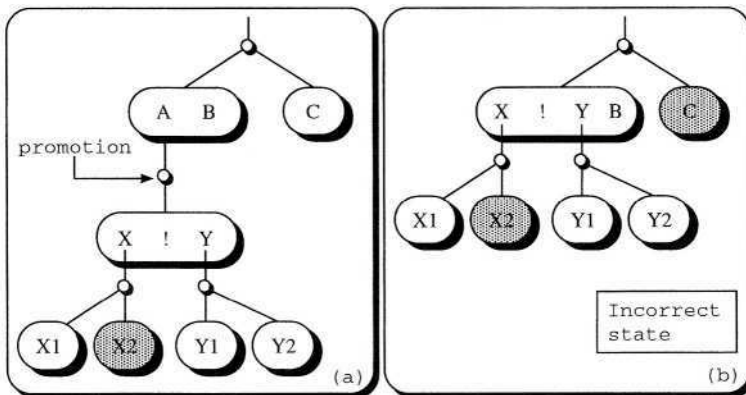
Fig. 10. Incorrect use of promotion and cut.
