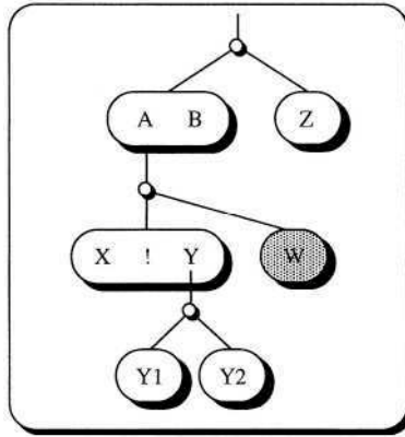
Fig. 9. Cut in the leftmost box in the tree.
