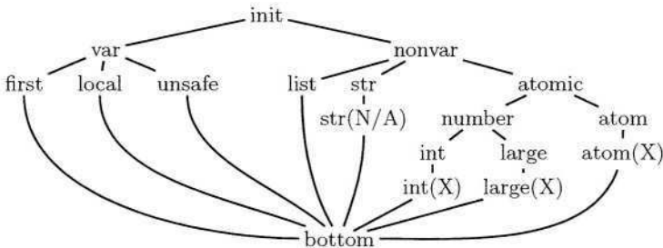
Fig. 6. Extended init subdomain.
