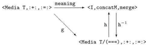
Fig. 1. The Structure of Interpretation
