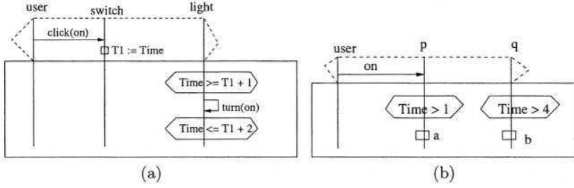
Fig. 6. (a) LSC with timing constraints (b) Choice in evaluating timing constraints
