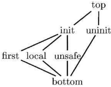
Fig. 1. Lattice of WAM types.
