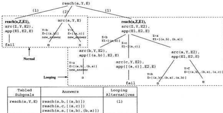
Fig. 1. DRA Resolution with Mode Declaration
