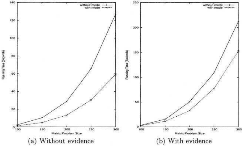
Fig. 3. Time Performance of Matrix-chain Multiplication
