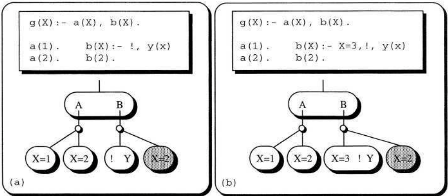
Fig. 7. Correct use of splitting and cut.
