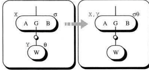
Fig. 2. BEAM promotion rule.
