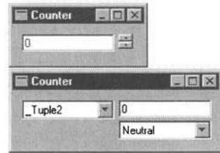
Fig.2. Two GEC_{Counter} s created by selfGEC updCntr (0, Neutral) . The standard one (bottom) and a customized one (top).
